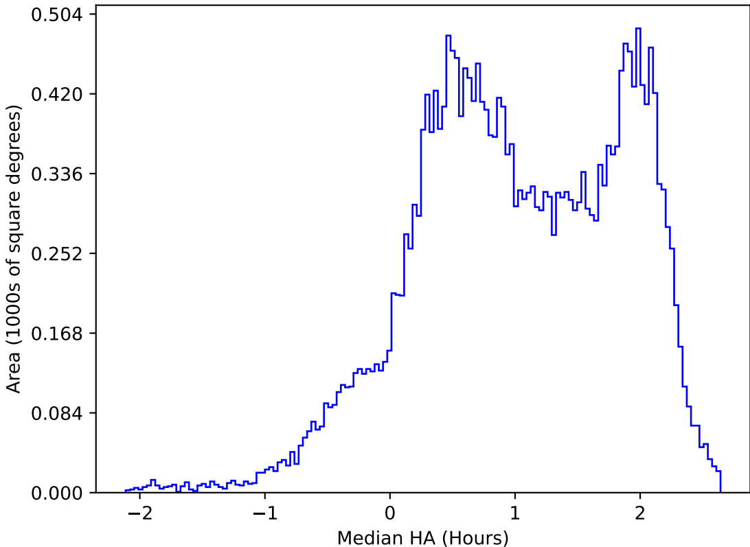
too_elab_r64_d3_ugrizy_v3.4_10yrs All sky z band: Median HA
