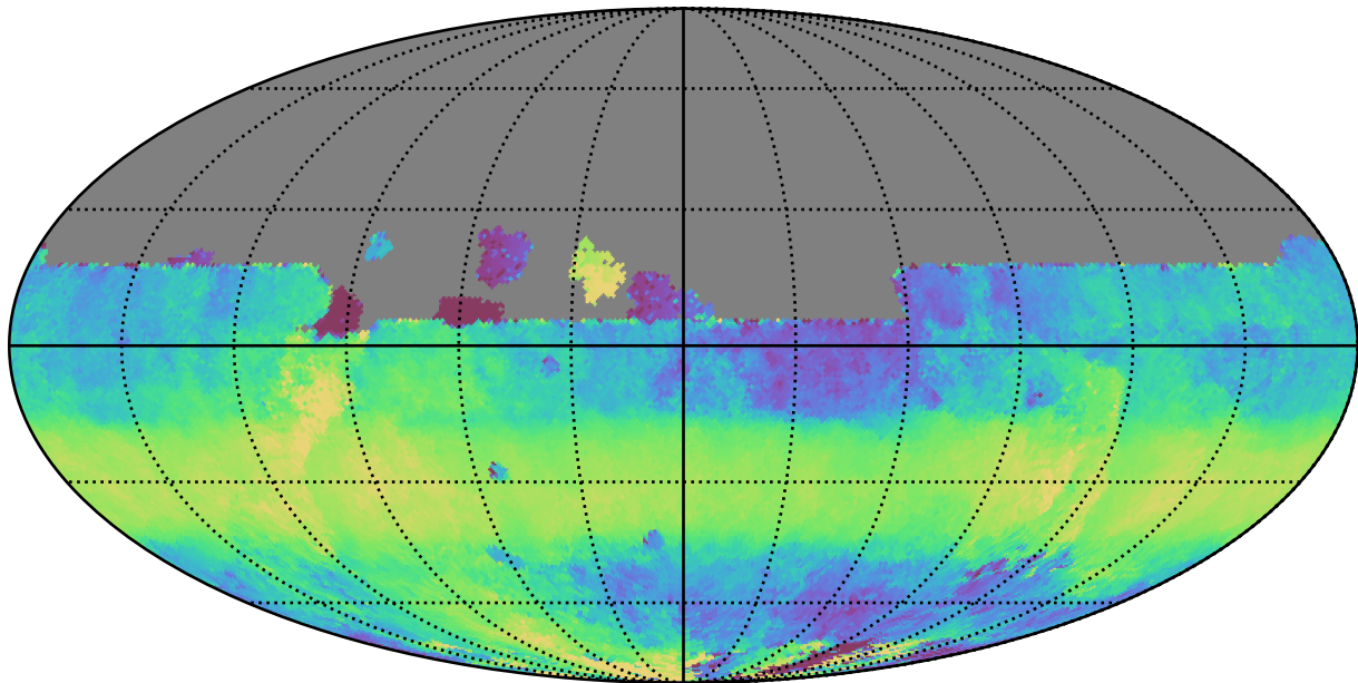
too_elab_r64_d3_ugrizy_v3.4_10yrs All sky y band: Median HA
