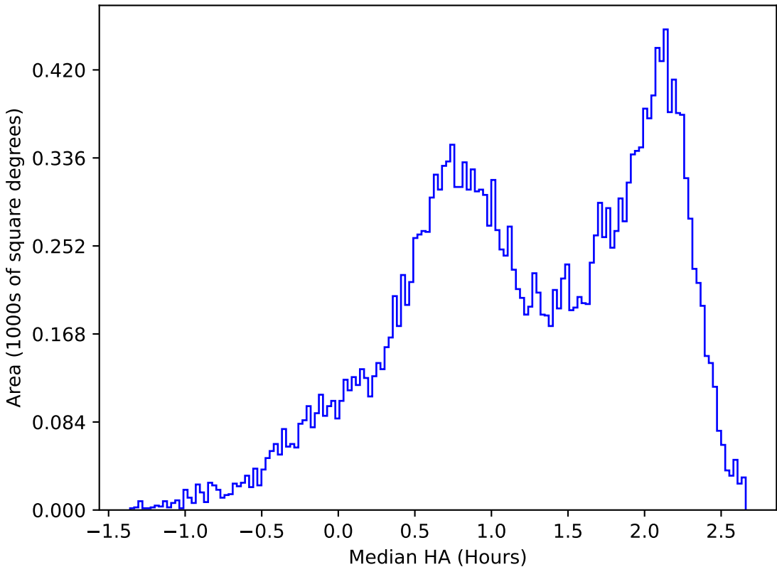
too_elab_r64_d3_ugrizy_v3.4_10yrs All sky y band: Median HA
