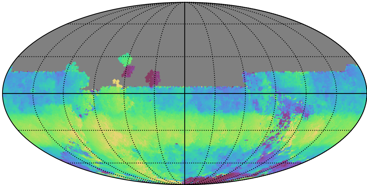
too_elab_r64_d3_ugrizy_v3.4_10yrs All sky u band: Median HA
