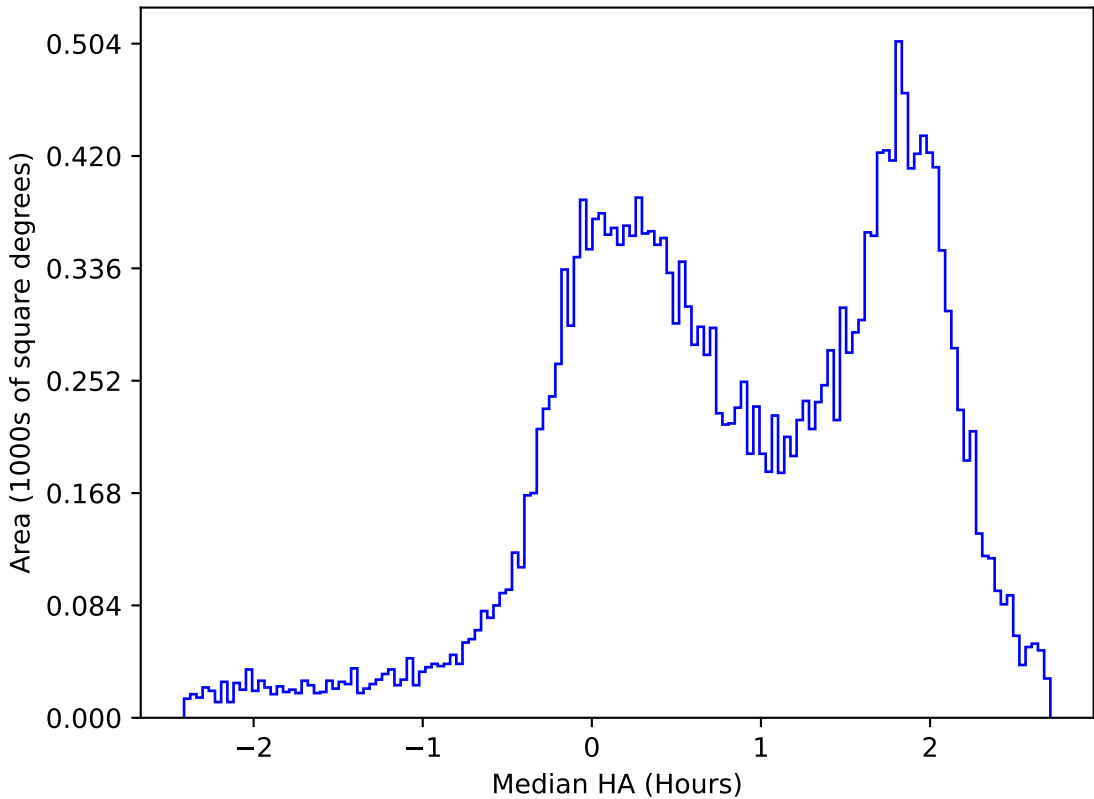
too_elab_r64_d3_ugrizy_v3.4_10yrs All sky u band: Median HA
