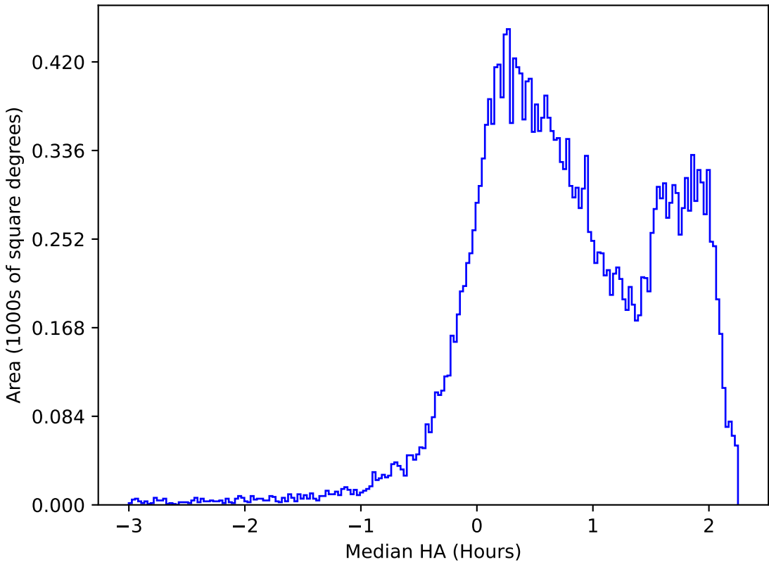
too_elab_r64_d3_ugrizy_v3.4_10yrs All sky r band: Median HA
