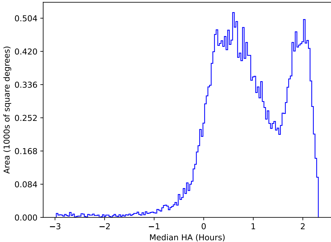
too_elab_r64_d3_ugrizy_v3.4_10yrs All sky i band: Median HA
