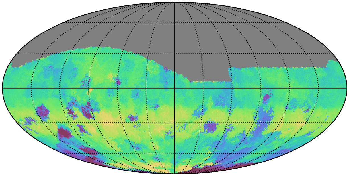
too_elab_r64_d3_ugrizy_v3.4_10yrs All sky g band: Median HA
