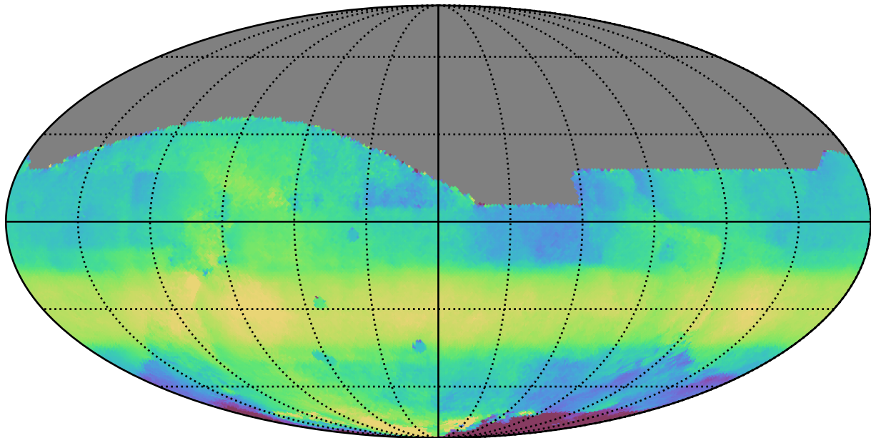
too_elab_r64_d3_ugrizy_v3.4_10yrs All sky all bands: Median HA
