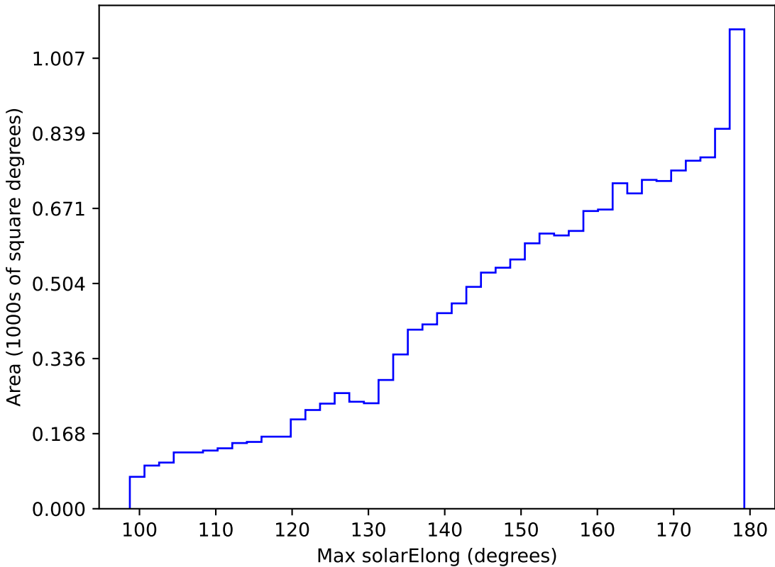
too_elab_r64_d3_ugrizy_v3.4_10yrs WFD z band: Max solarElong
