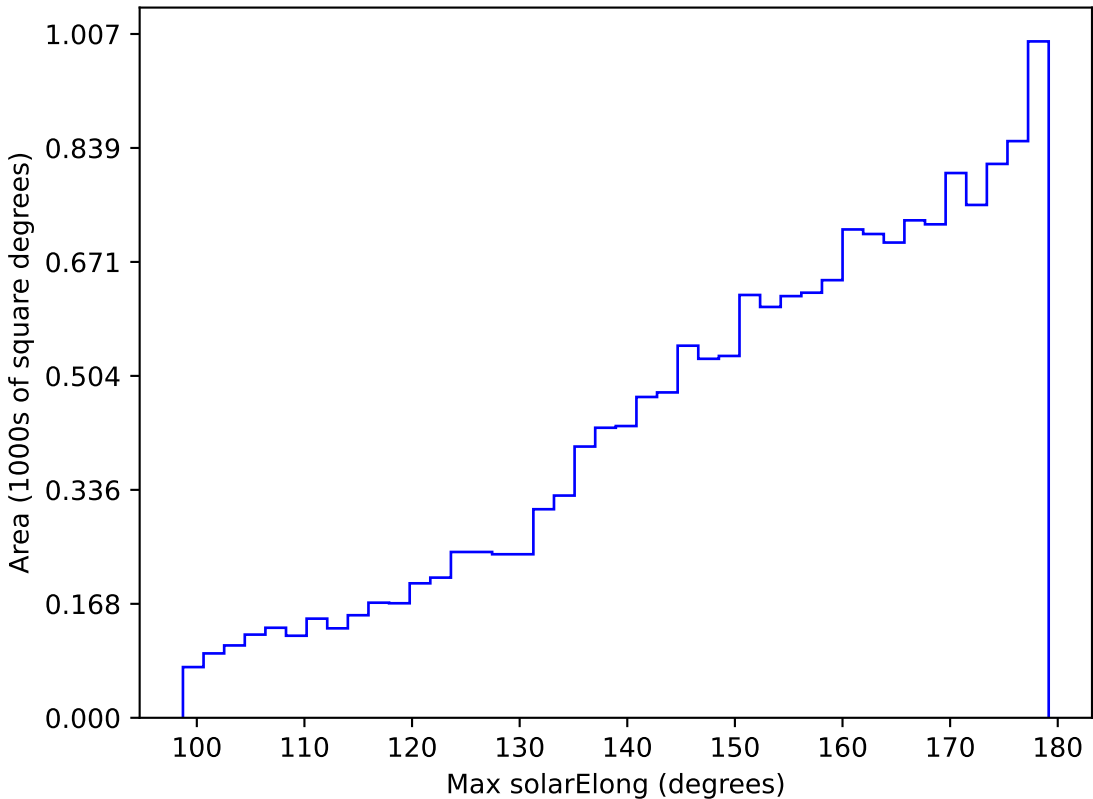
too_elab_r64_d3_ugrizy_v3.4_10yrs WFD y band: Max solarElong
