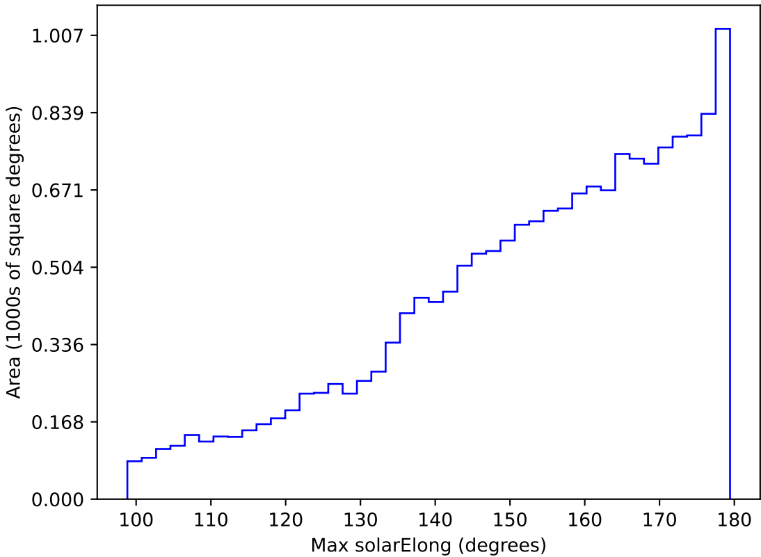
too_elab_r64_d3_ugrizy_v3.4_10yrs WFD r band: Max solarElong
