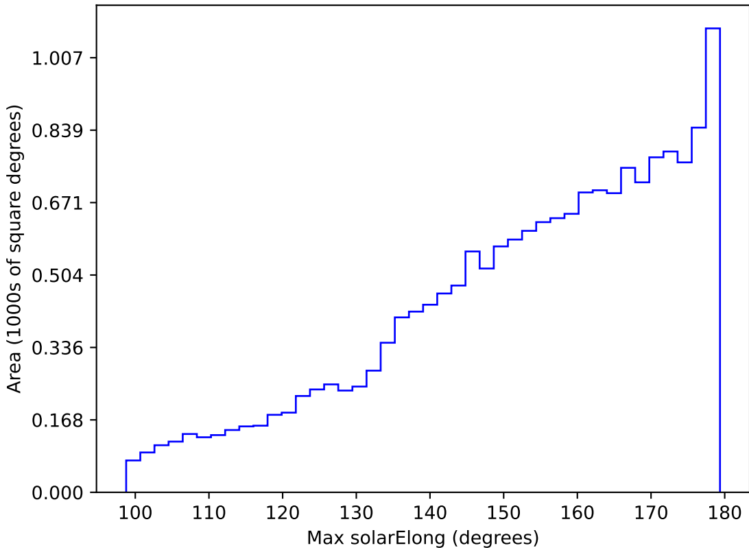
too_elab_r64_d3_ugrizy_v3.4_10yrs WFD i band: Max solarElong
