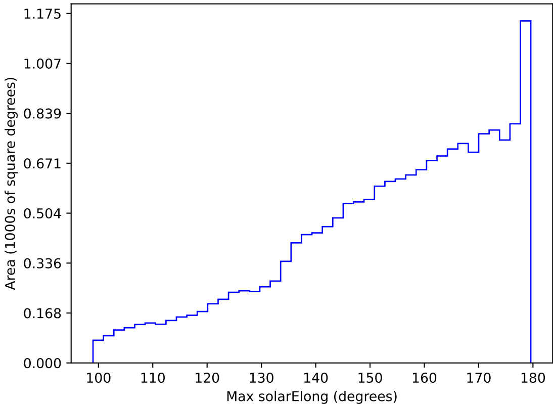
too_elab_r64_d3_ugrizy_v3.4_10yrs WFD all bands: Max solarElong
