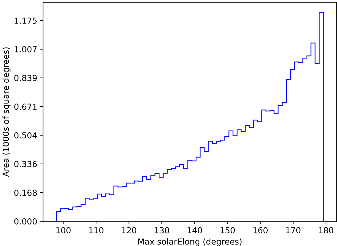
too_elab_r64_d3_ugrizy_v3.4_10yrs All sky z band: Max solarElong
