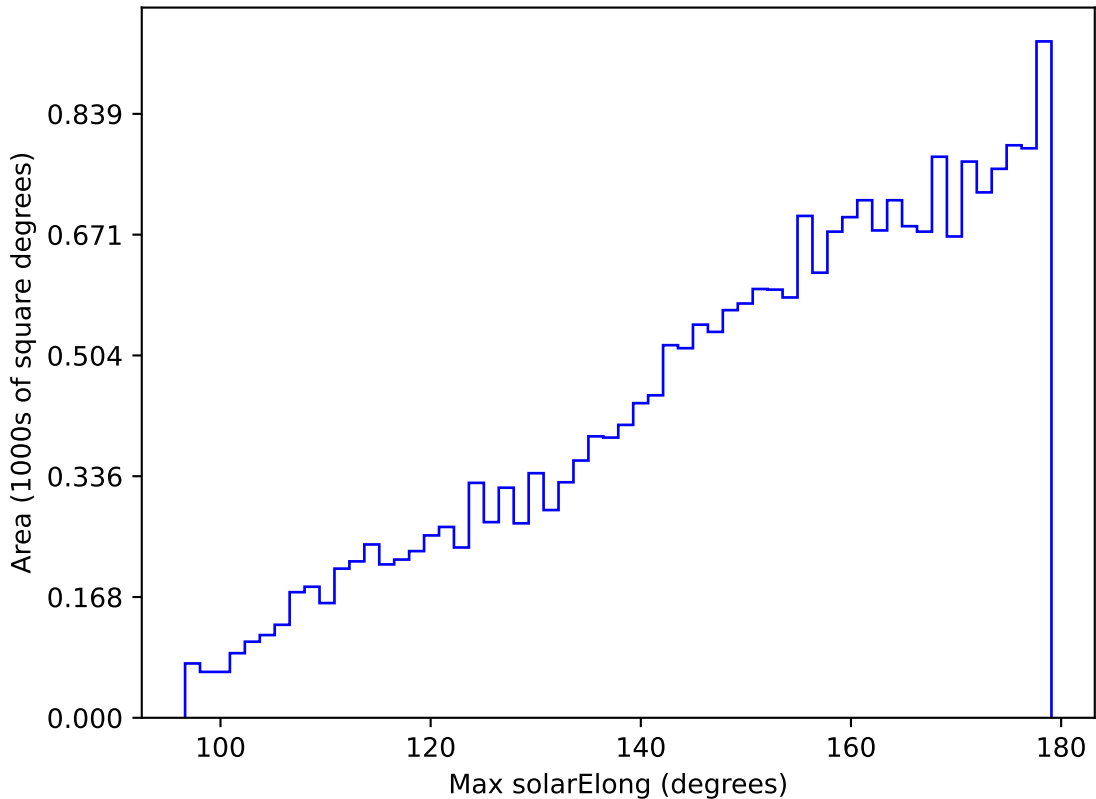
too_elab_r64_d3_ugrizy_v3.4_10yrs All sky y band: Max solarElong
