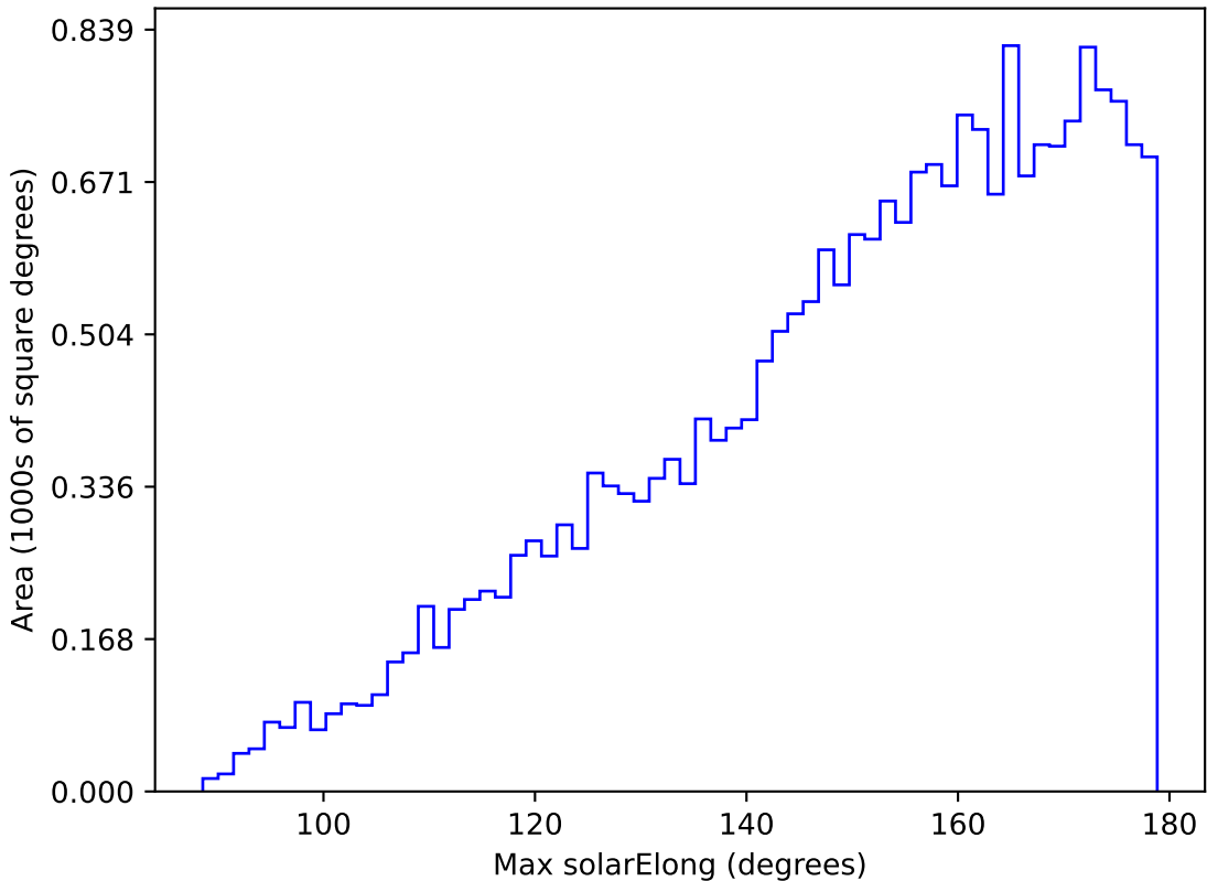
too_elab_r64_d3_ugrizy_v3.4_10yrs All sky u band: Max solarElong
