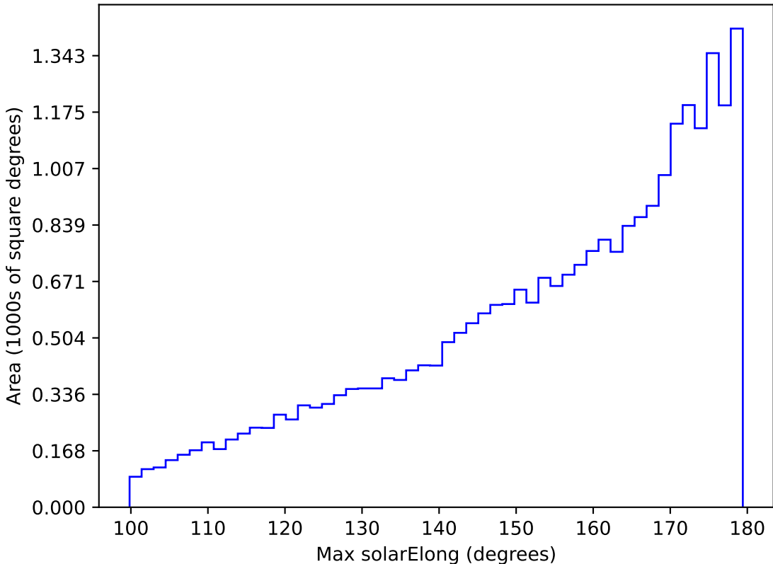
too_elab_r64_d3_ugrizy_v3.4_10yrs All sky r band: Max solarElong
