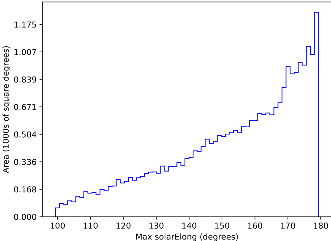
too_elab_r64_d3_ugrizy_v3.4_10yrs All sky i band: Max solarElong
