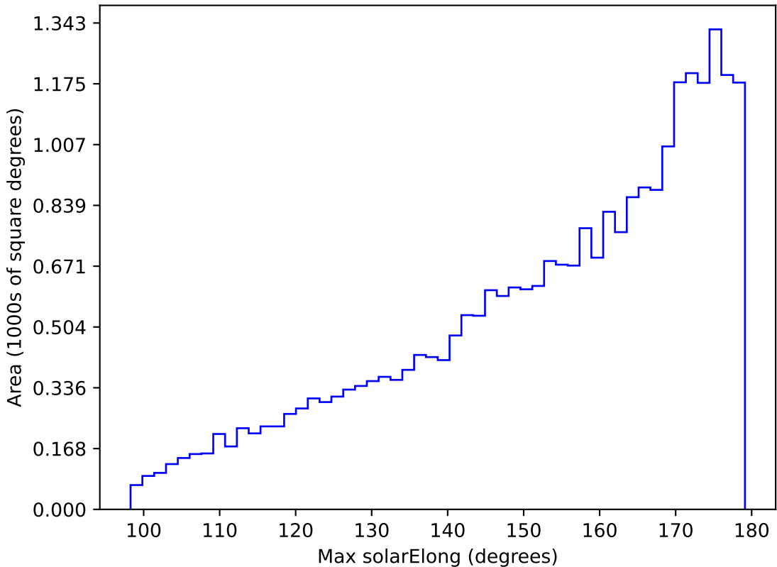
too_elab_r64_d3_ugrizy_v3.4_10yrs All sky g band: Max solarElong
