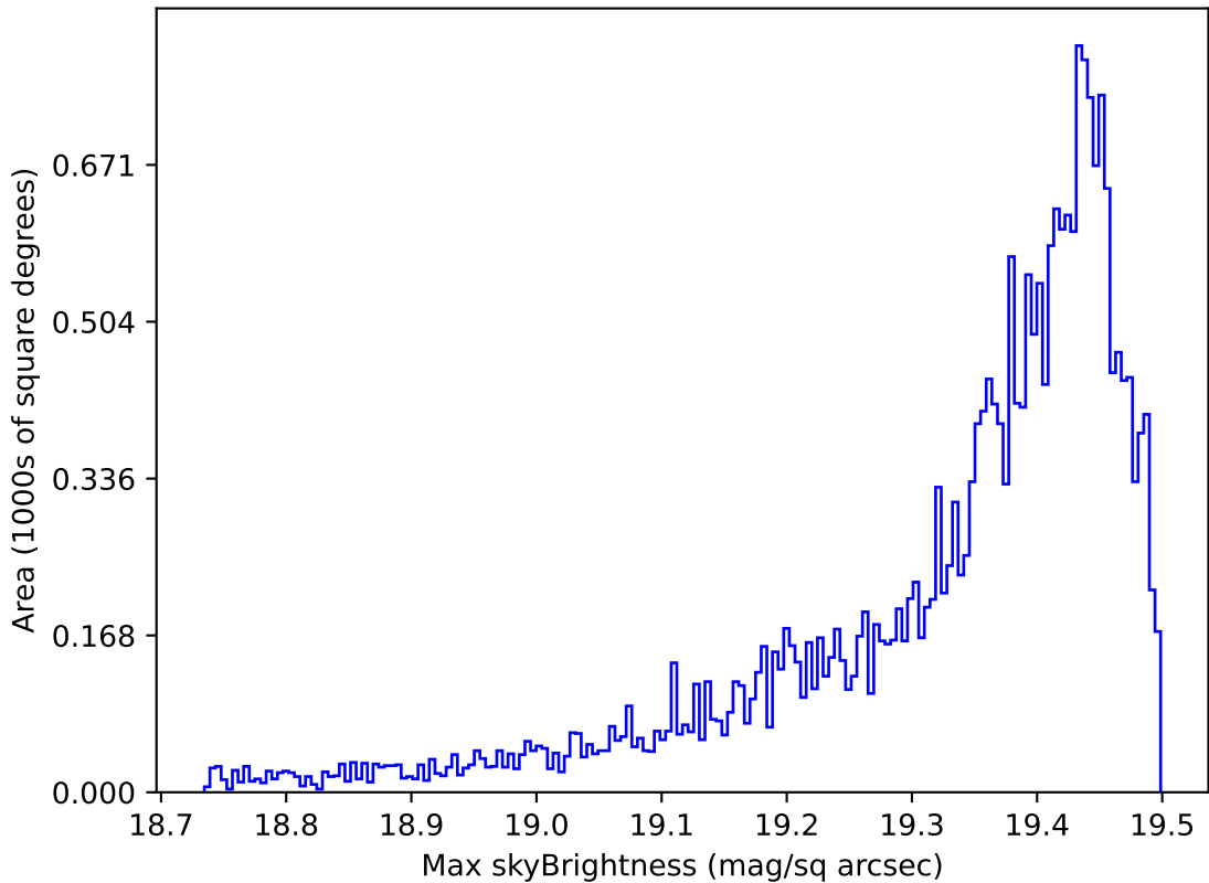
too_elab_r64_d3_ugrizy_v3.4_10yrs Yr 1 z band: Max skyBrightness
