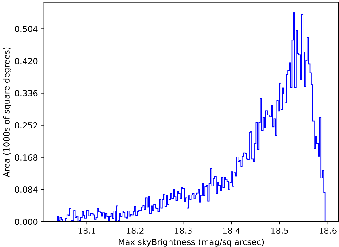
too_elab_r64_d3_ugrizy_v3.4_10yrs Yr 1 y band: Max skyBrightness
