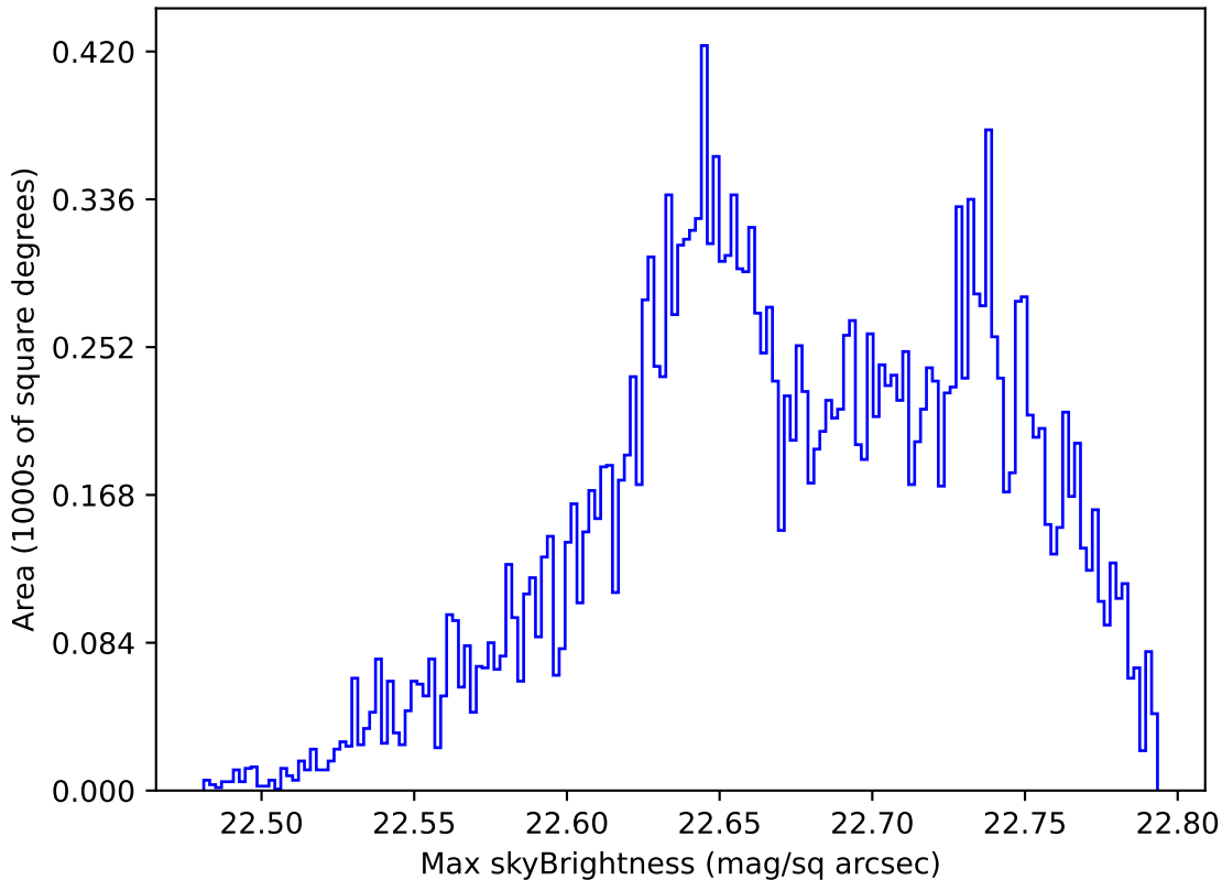
too_elab_r64_d3_ugrizy_v3.4_10yrs Yr 1 u band: Max skyBrightness
