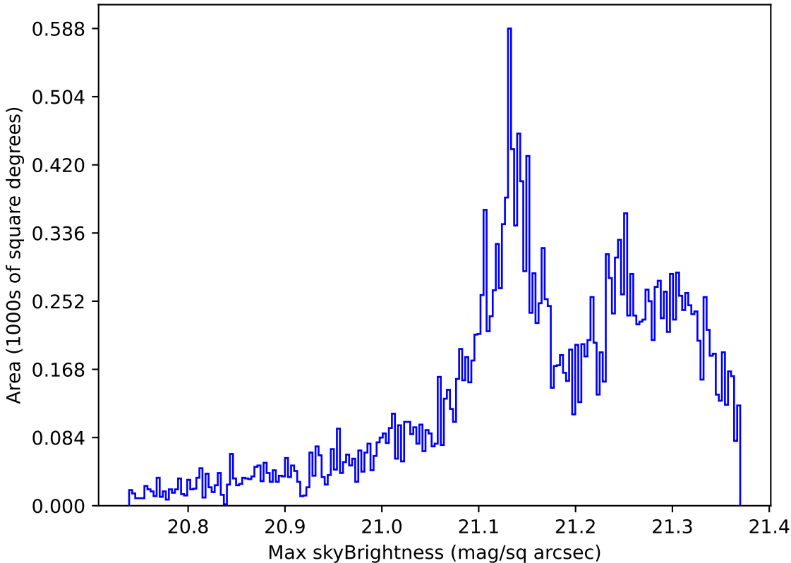
too_elab_r64_d3_ugrizy_v3.4_10yrs Yr 1 r band: Max skyBrightness
