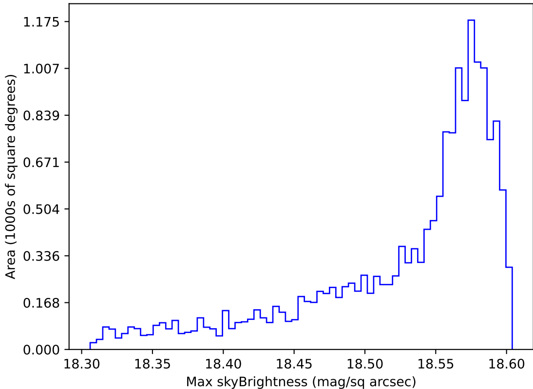
too_elab_r64_d3_ugrizy_v3.4_10yrs WFD y band: Max skyBrightness
