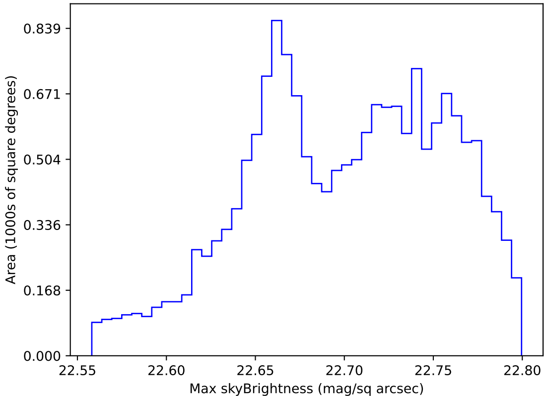
too_elab_r64_d3_ugrizy_v3.4_10yrs WFD u band: Max skyBrightness
