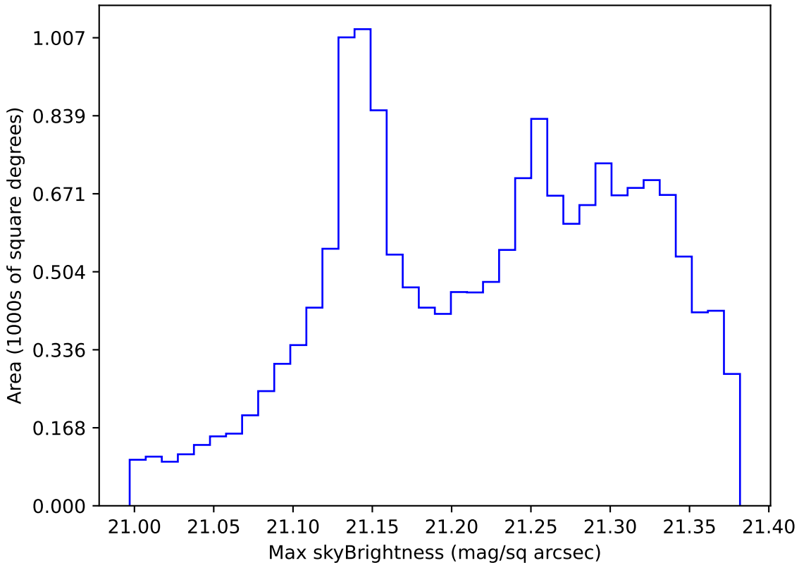
too_elab_r64_d3_ugrizy_v3.4_10yrs WFD r band: Max skyBrightness
