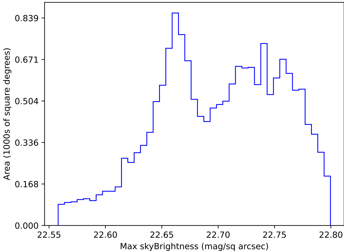
too_elab_r64_d3_ugrizy_v3.4_10yrs WFD all bands: Max skyBrightness
