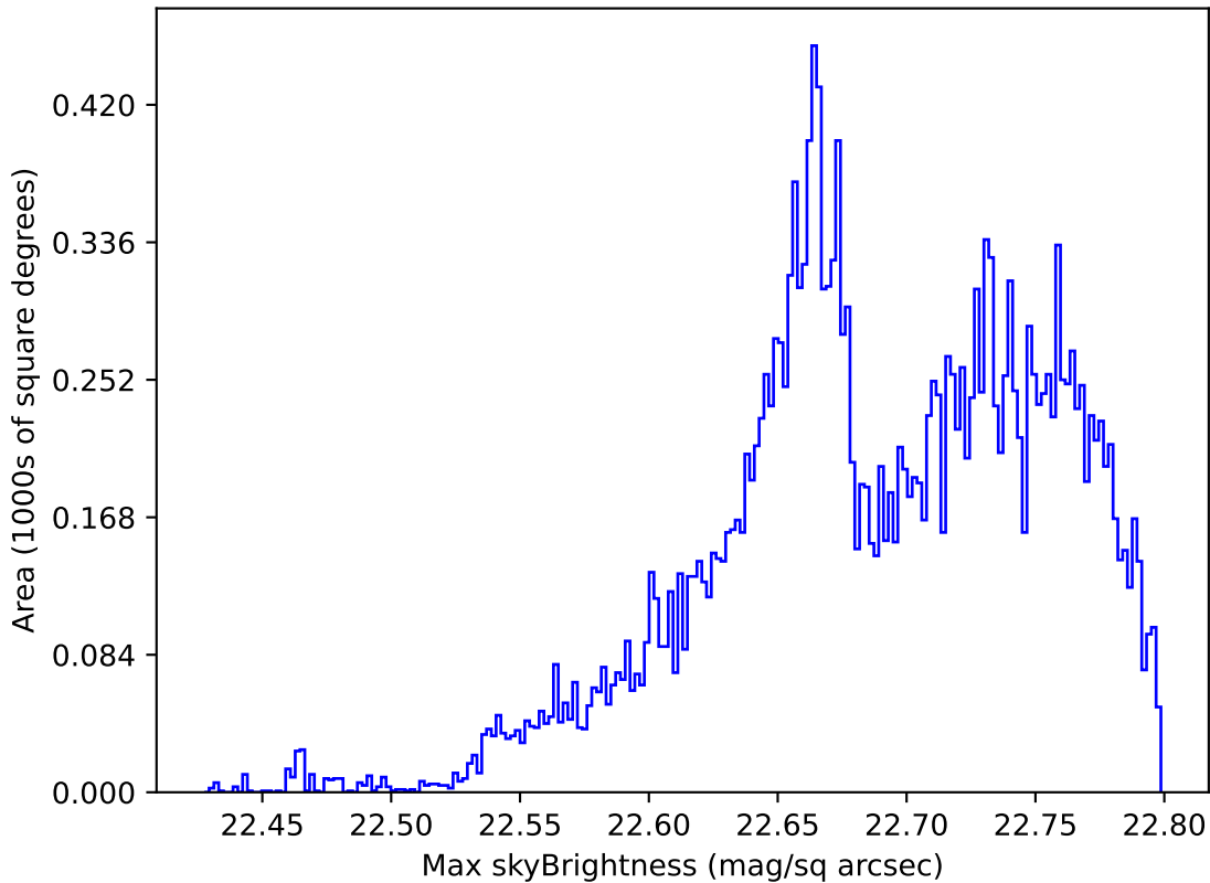
too_elab_r64_d3_ugrizy_v3.4_10yrs All sky u band: Max skyBrightness
