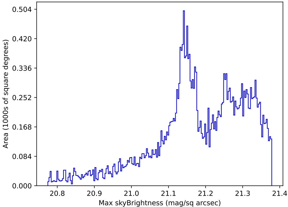
too_elab_r64_d3_ugrizy_v3.4_10yrs All sky r band: Max skyBrightness
