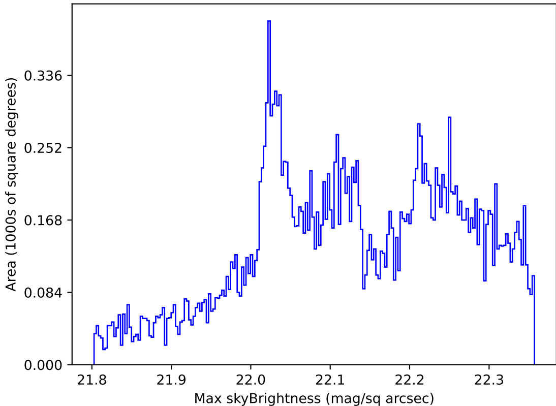
too_elab_r64_d3_ugrizy_v3.4_10yrs All sky g band: Max skyBrightness
