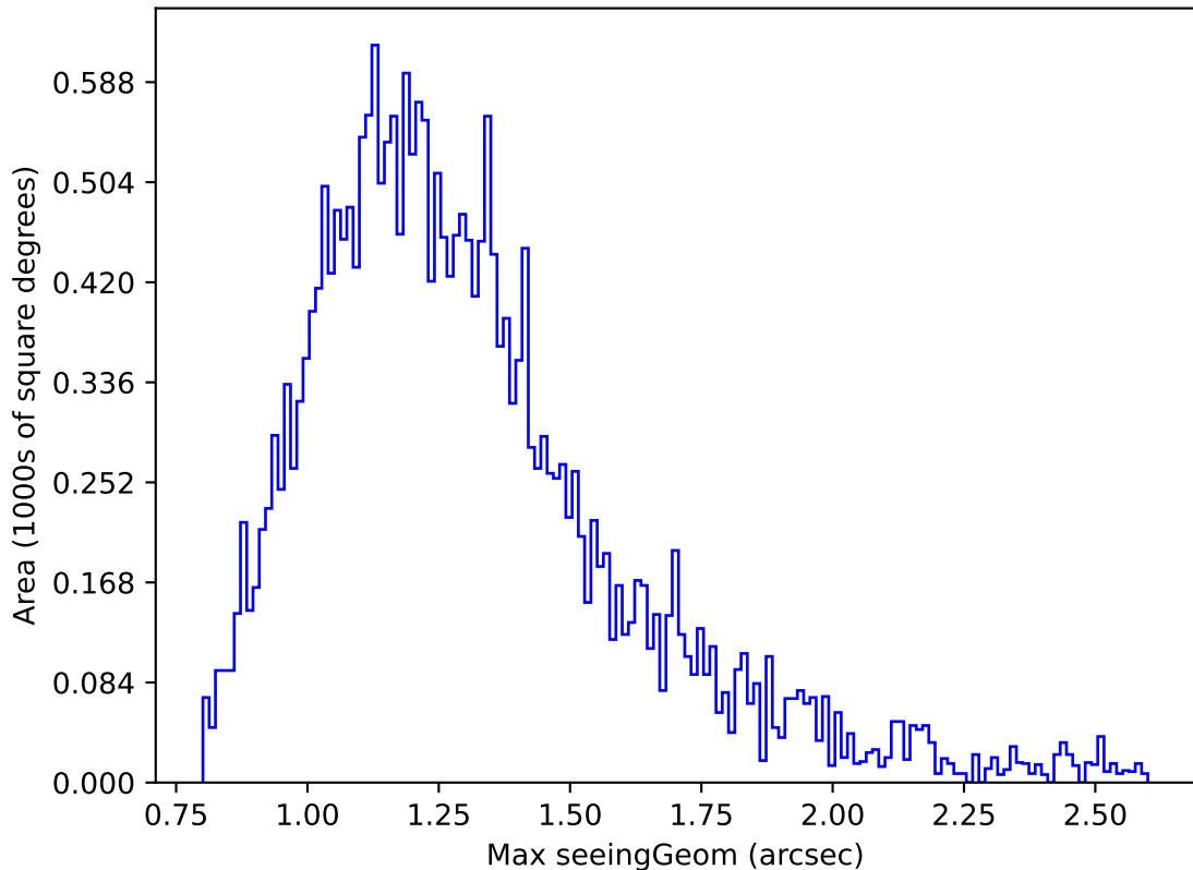
too_elab_r64_d3_ugrizy_v3.4_10yrs Yr 1 z band: Max seeingGeom
