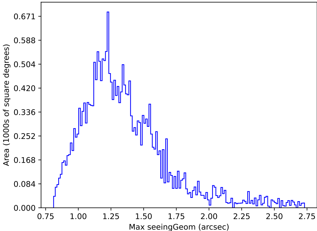
too_elab_r64_d3_ugrizy_v3.4_10yrs Yr 1 u band: Max seeingGeom
