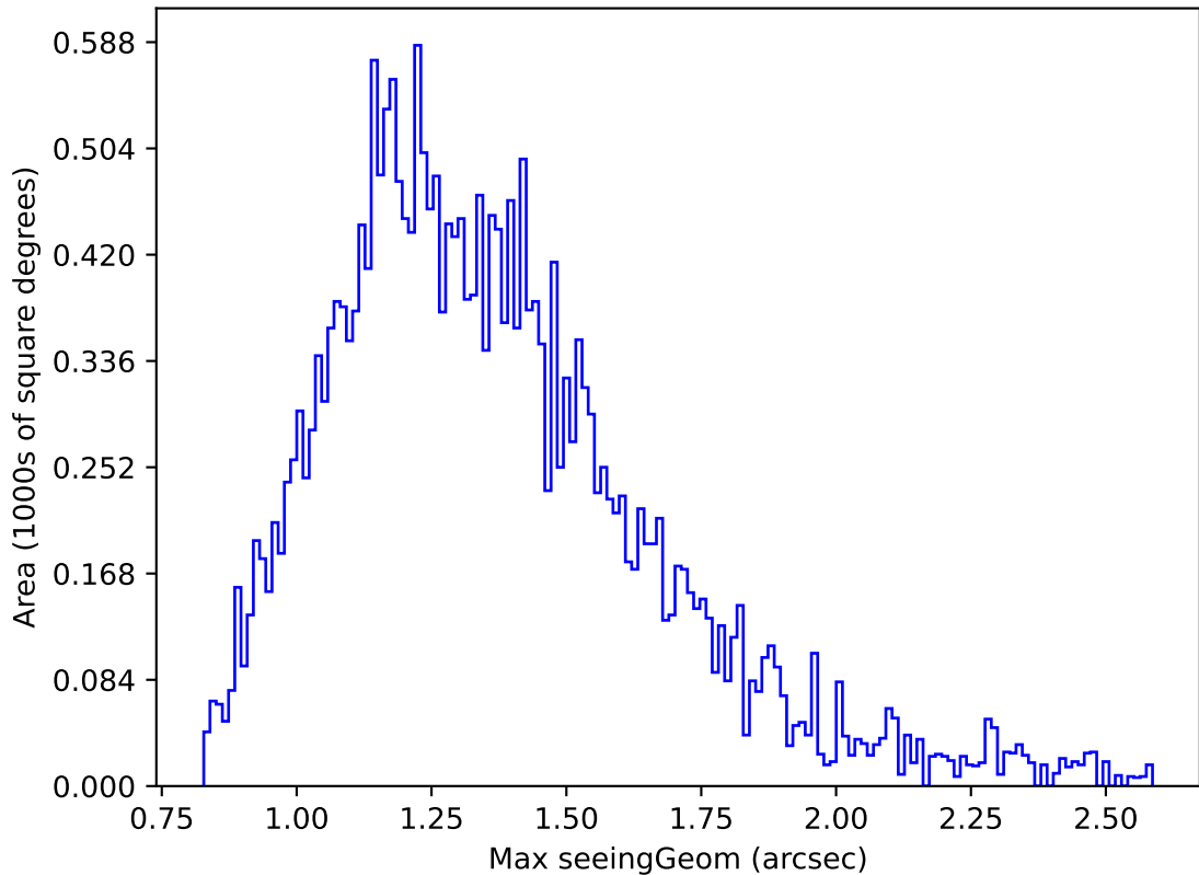
too_elab_r64_d3_ugrizy_v3.4_10yrs Yr 1 i band: Max seeingGeom
