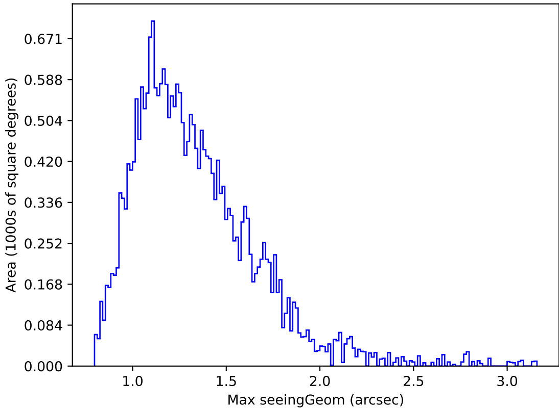
too_elab_r64_d3_ugrizy_v3.4_10yrs Yr 1 g band: Max seeingGeom
