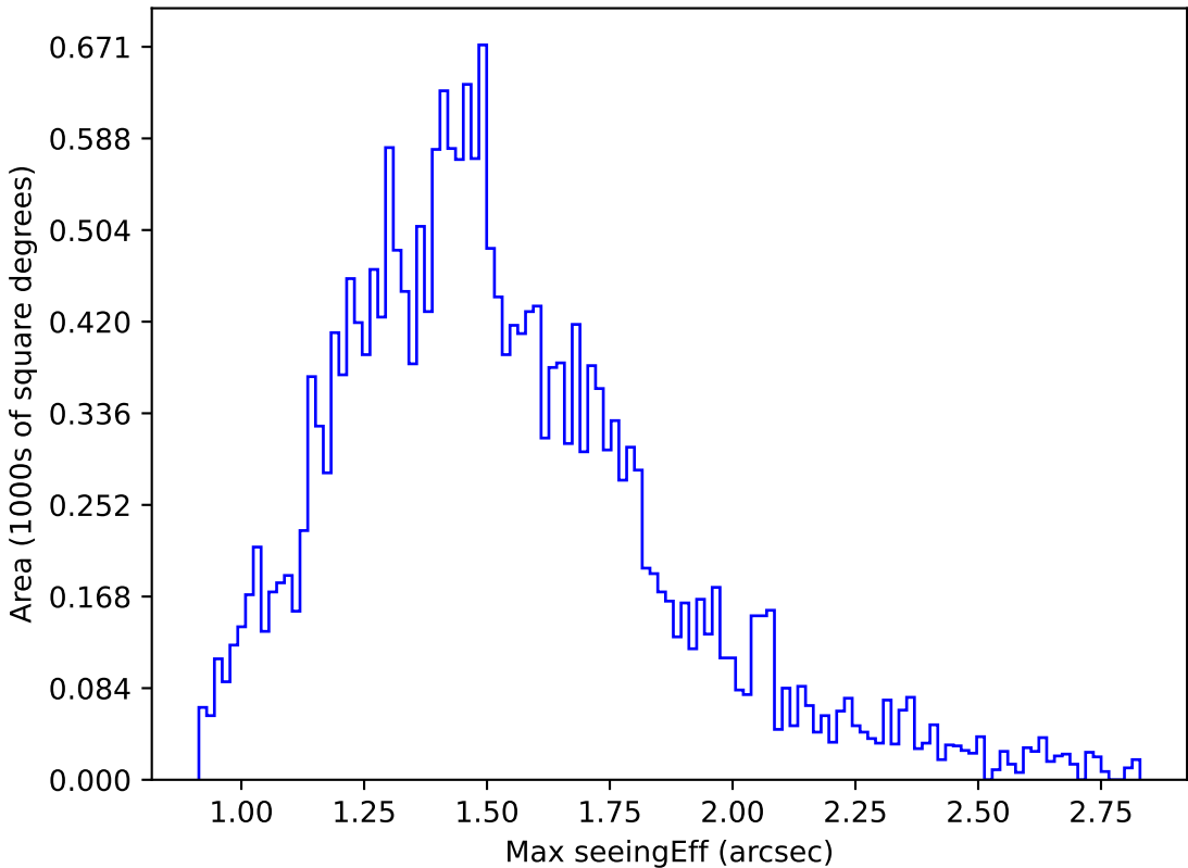
too_elab_r64_d3_ugrizy_v3.4_10yrs Yr 1 y band: Max seeingEff
