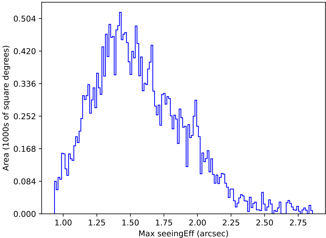
too_elab_r64_d3_ugrizy_v3.4_10yrs Yr 1 r band: Max seeingEff
