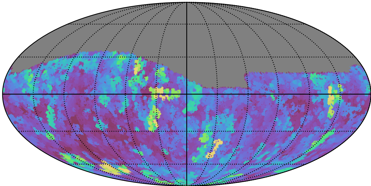
too_elab_r64_d3_ugrizy_v3.4_10yrs Yr 1 i band: Max seeingEff
