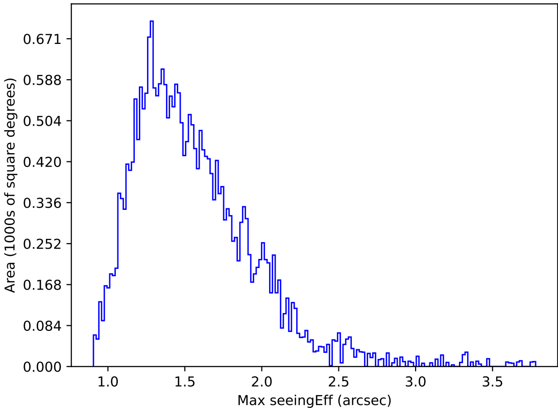
too_elab_r64_d3_ugrizy_v3.4_10yrs Yr 1 g band: Max seeingEff
