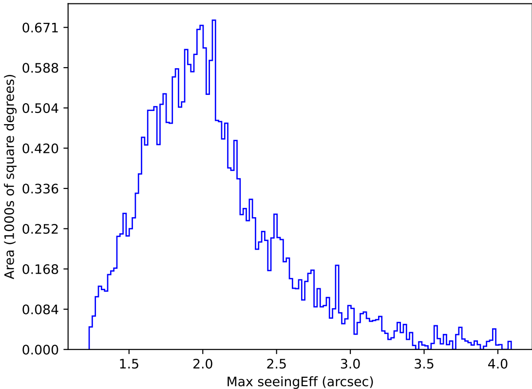
too_elab_r64_d3_ugrizy_v3.4_10yrs Yr 1 all bands: Max seeingEff
