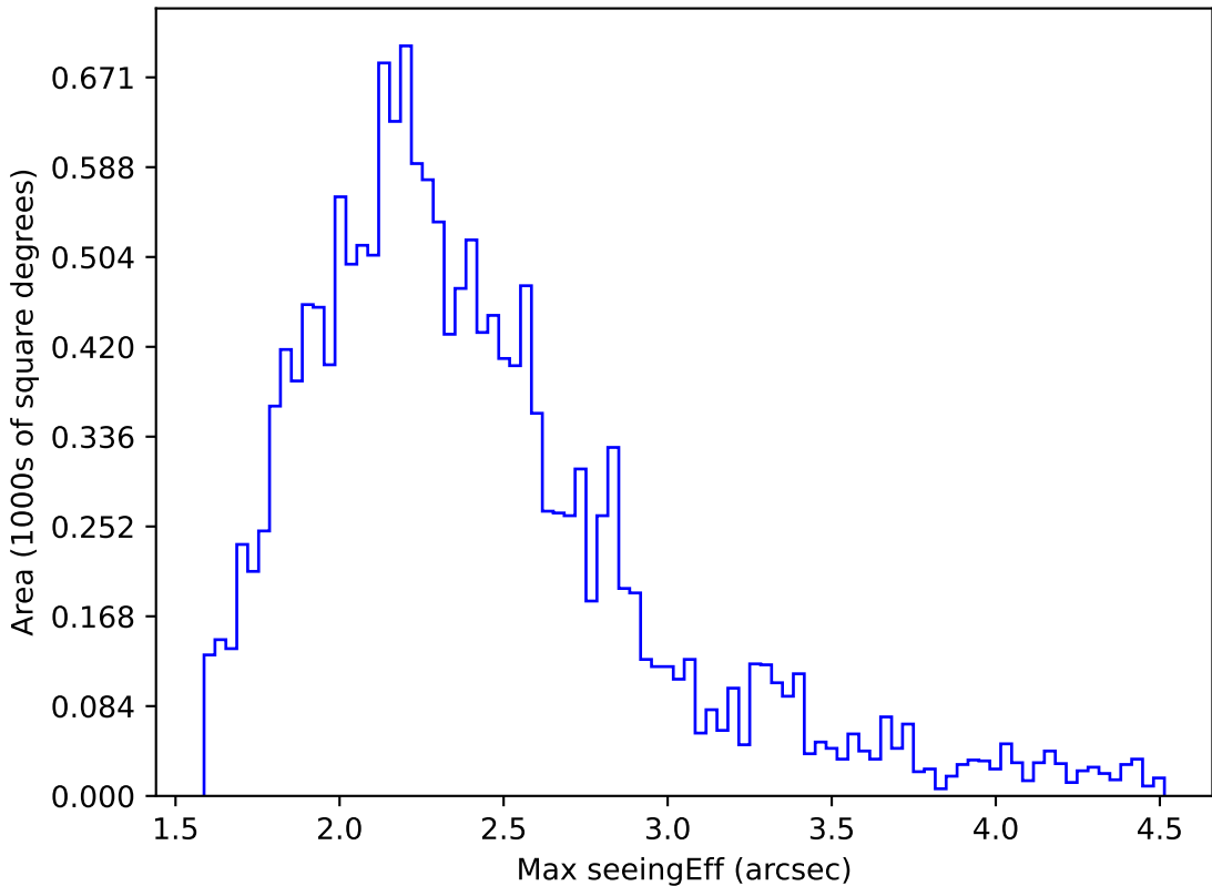
too_elab_r64_d3_ugrizy_v3.4_10yrs WFD y band: Max seeingEff
