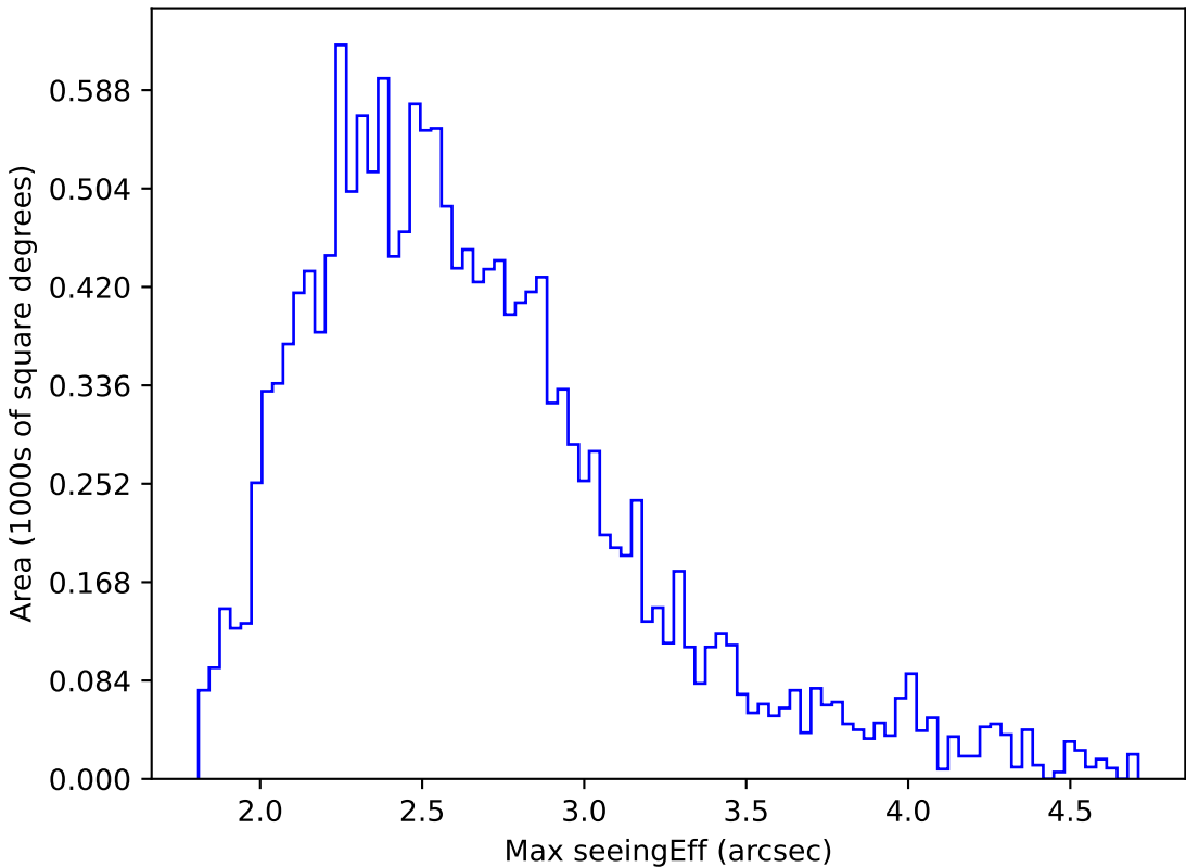
too_elab_r64_d3_ugrizy_v3.4_10yrs WFD r band: Max seeingEff
