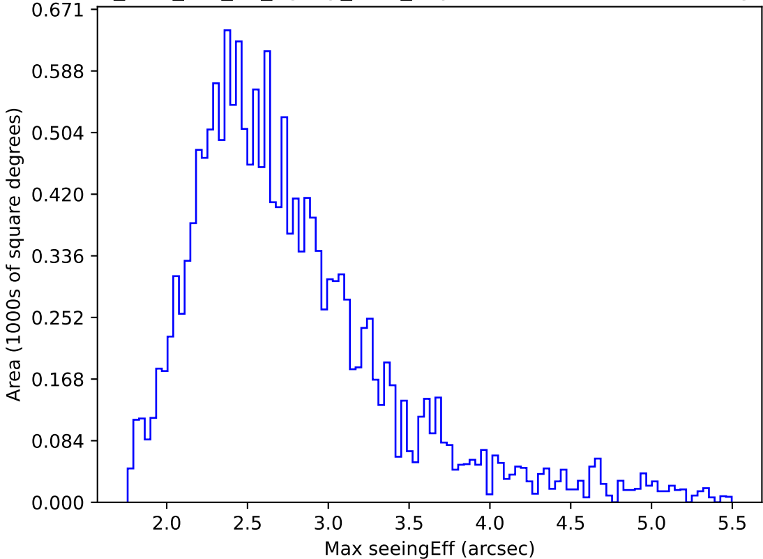
too_elab_r64_d3_ugrizy_v3.4_10yrs WFD i band: Max seeingEff
