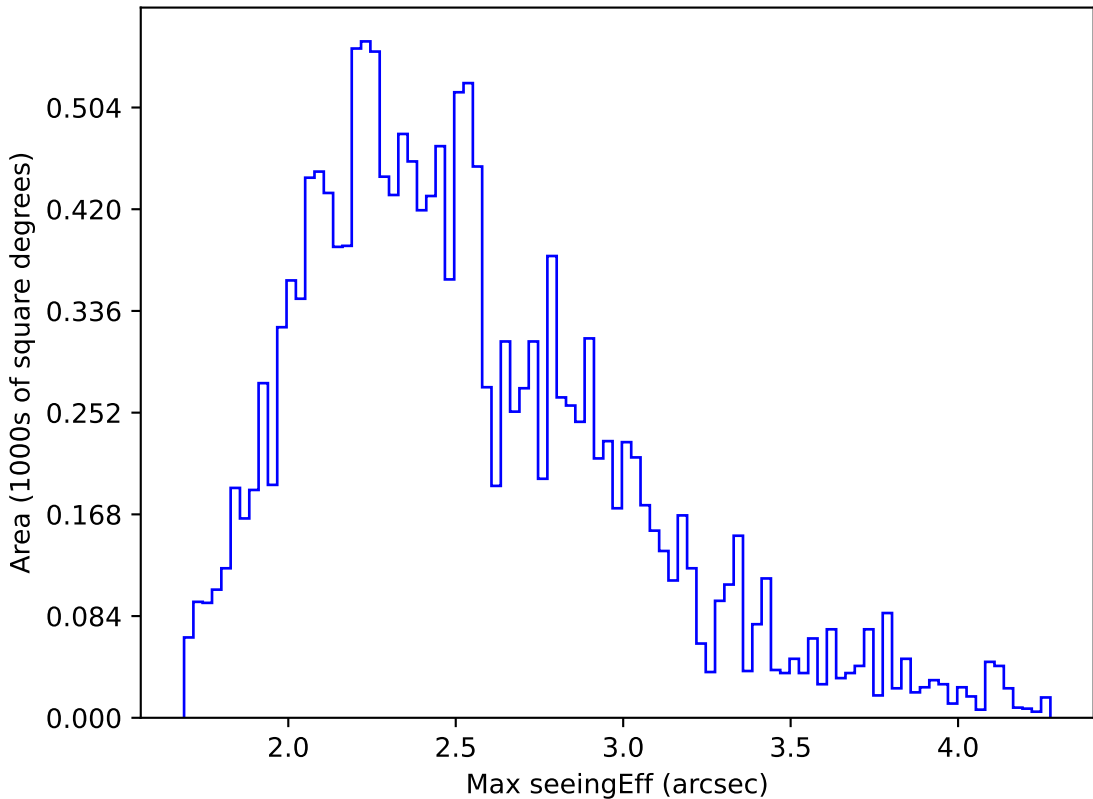
too_elab_r64_d3_ugrizy_v3.4_10yrs WFD g band: Max seeingEff
