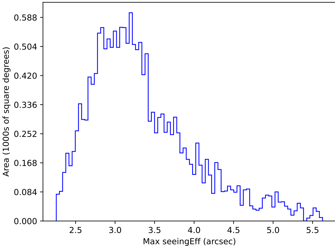
too_elab_r64_d3_ugrizy_v3.4_10yrs WFD all bands: Max seeingEff
