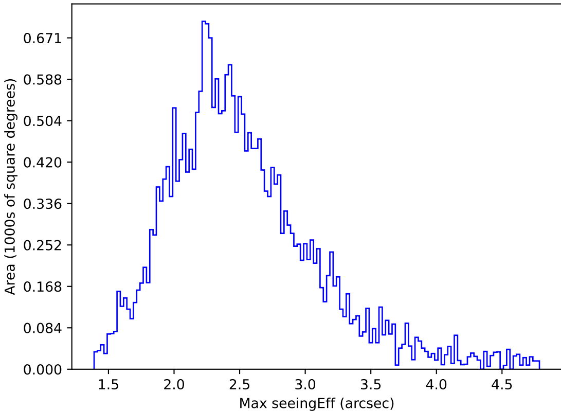
too_elab_r64_d3_ugrizy_v3.4_10yrs All sky z band: Max seeingEff
