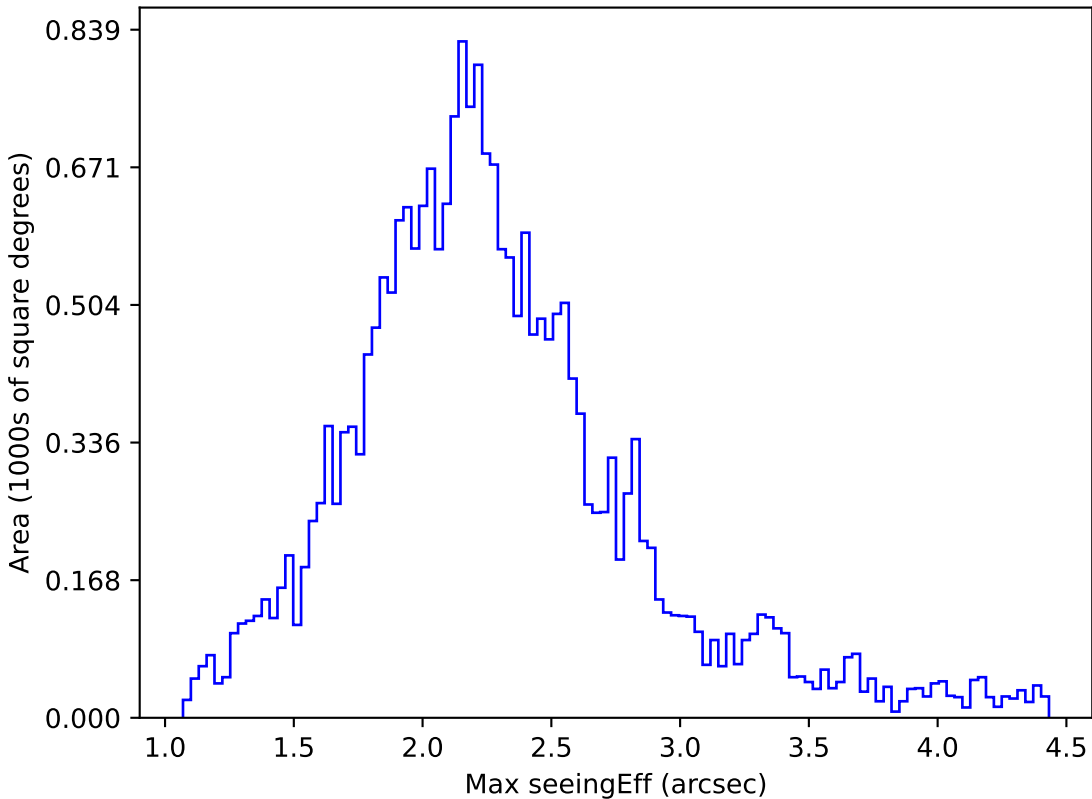
too_elab_r64_d3_ugrizy_v3.4_10yrs All sky y band: Max seeingEff
