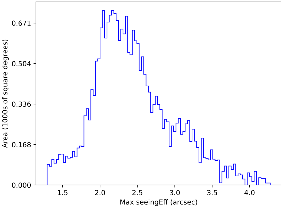
too_elab_r64_d3_ugrizy_v3.4_10yrs All sky u band: Max seeingEff
