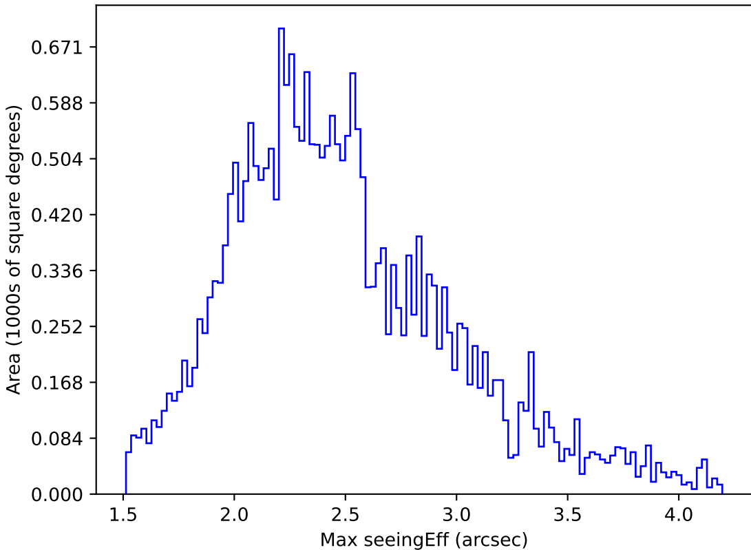
too_elab_r64_d3_ugrizy_v3.4_10yrs All sky g band: Max seeingEff
