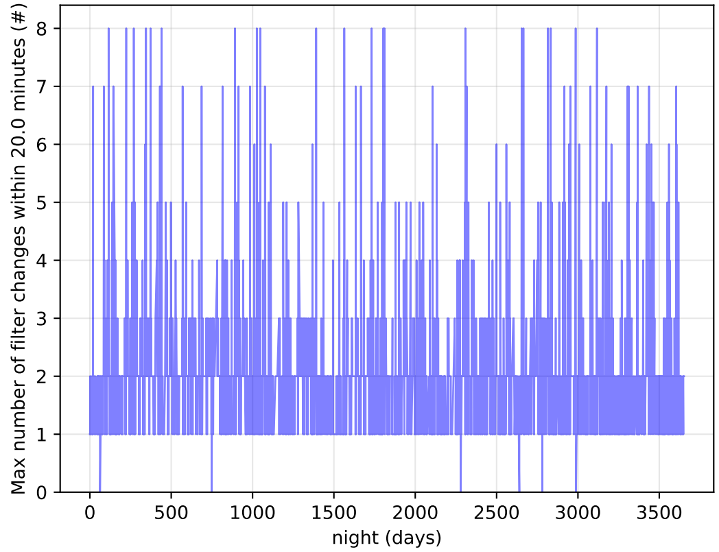
too_elab_r64_d3_ugrizyv3.4_10yrs Per Night: Max number of filter changes within 20.0 minutes
